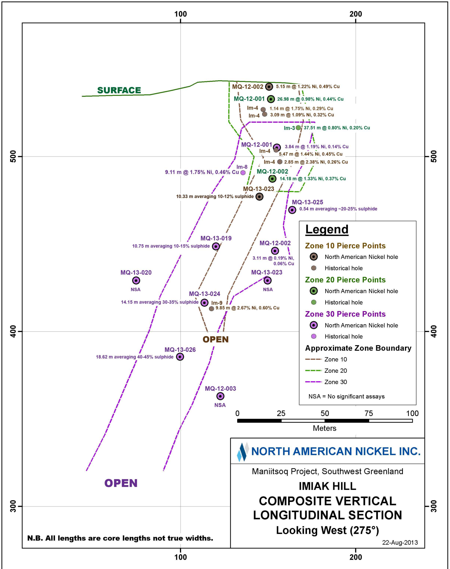
Figure 3: Imiak Composite Longitudinal Section
