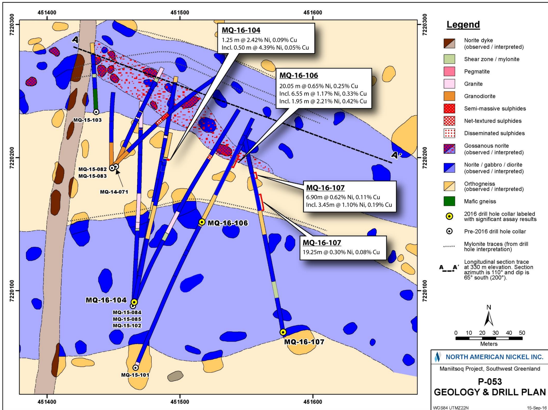
Figure 2: P-053 geology and drill plan.
