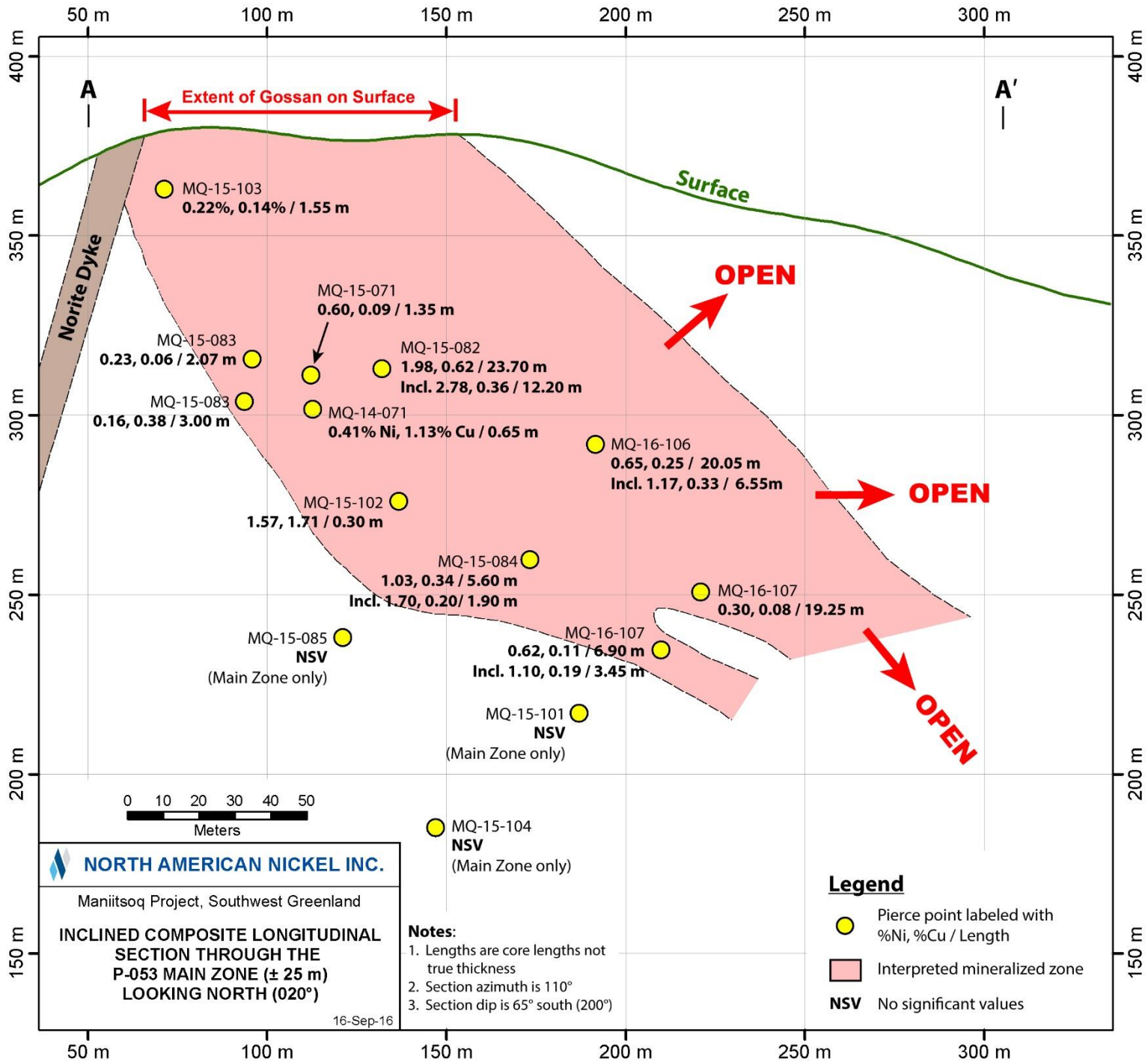
Figure 3: Composite included longitudinal section through the P-053 Main Zone. The azimuth of the section is 110° and it looks N020°E.
